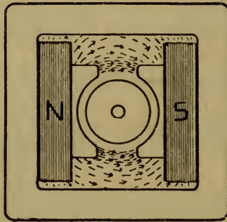
Figure 40 Magnetic leakage in internal pole bipolar frame.
